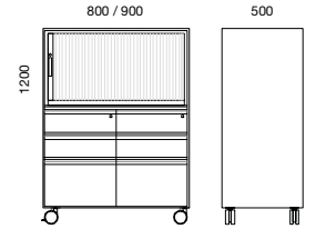
Lateral Docking Unit
