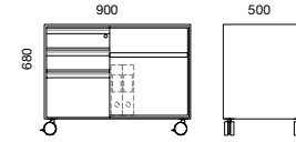
Combo Unit -BBF/Open
