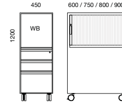
Vertical Docking Tower
